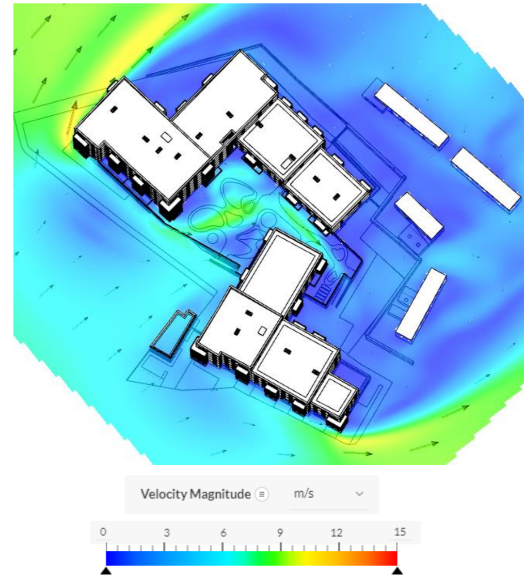
Fig 4.1 –Velocity Contours at 10m above Ground Level
