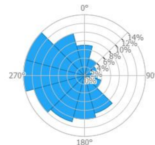
Fig 3.1.2 – Wind Frequency Rose for Castle Street – Global Wind Atlas
