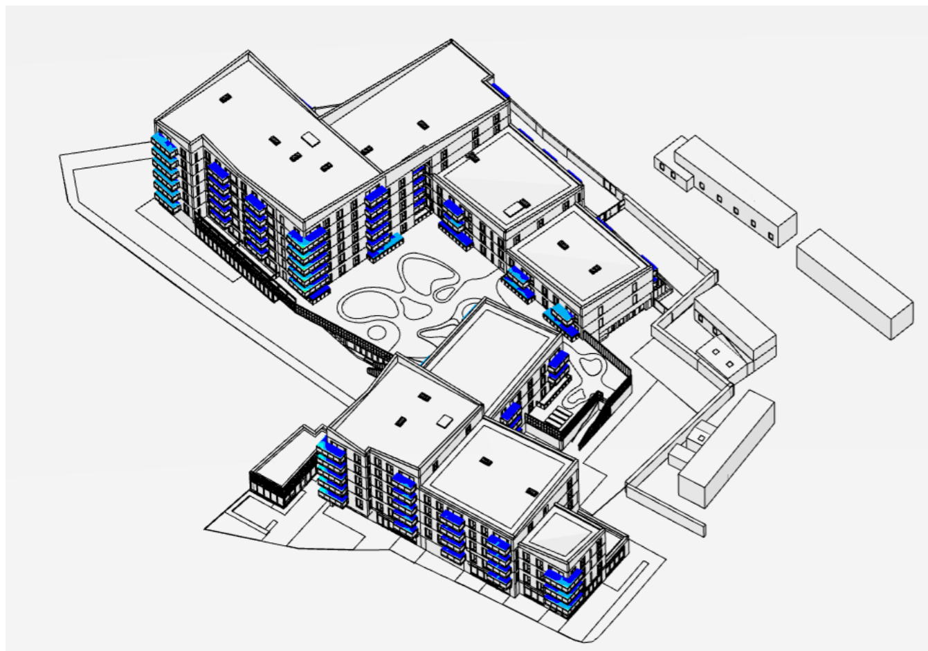
Fig 5.4.1 – Lawson Criteria Results for Balcony Levels - View from South
