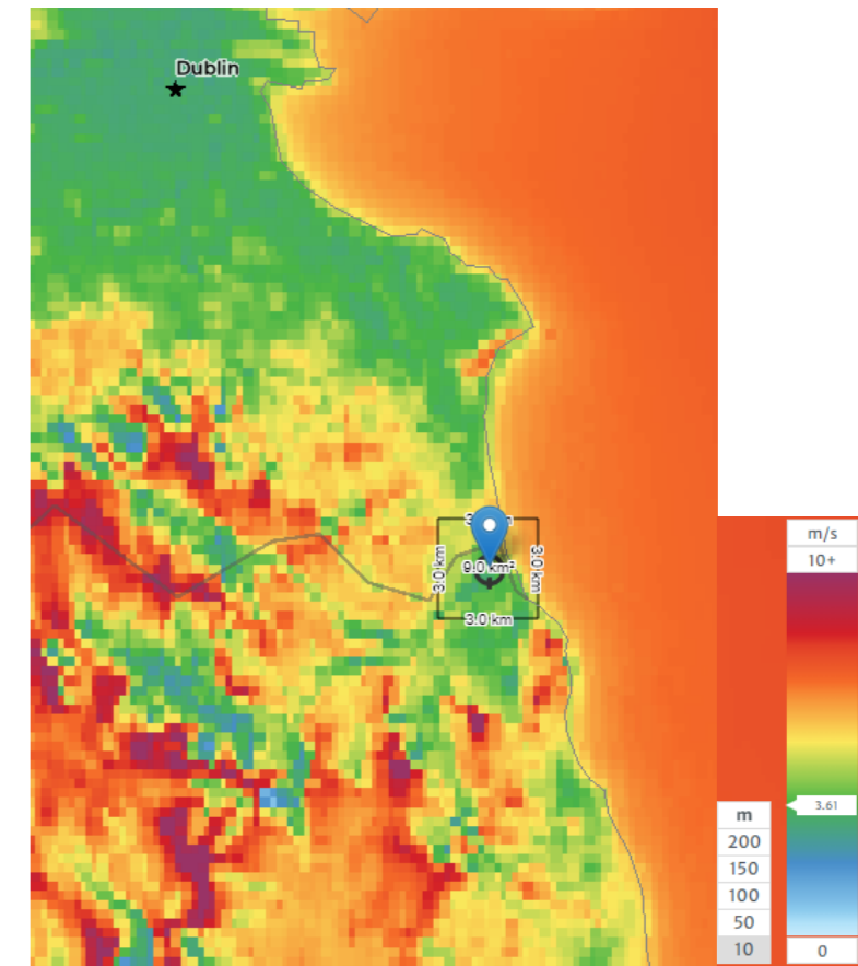
Fig 3.1.1 – Mean Wind Speeds at 10m above Ground across North Wicklow – Global Wind Atlas
