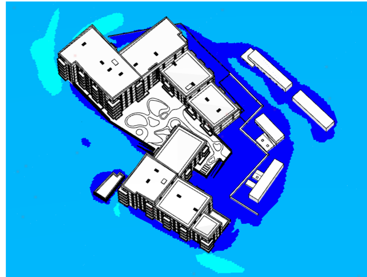
Fig 2.0 – Lawson Criteria Results Across Proposed Castle Street Development
