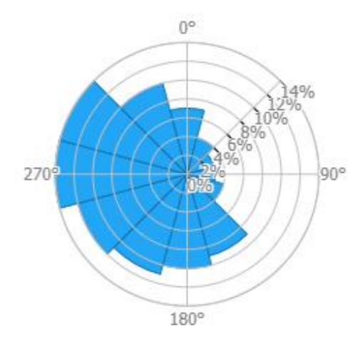
Fig 3.1.3 – Wind Speed Rose for Castle Street – Global Wind Atlas
