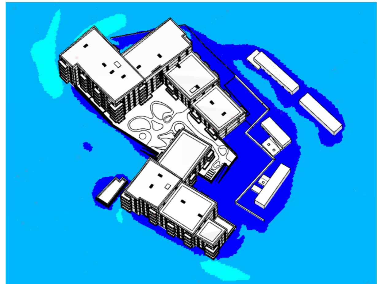
Fig 5.1 – Lawson Criteria Results at 1.5m above Ground Level across Proposed Castle Street Development
